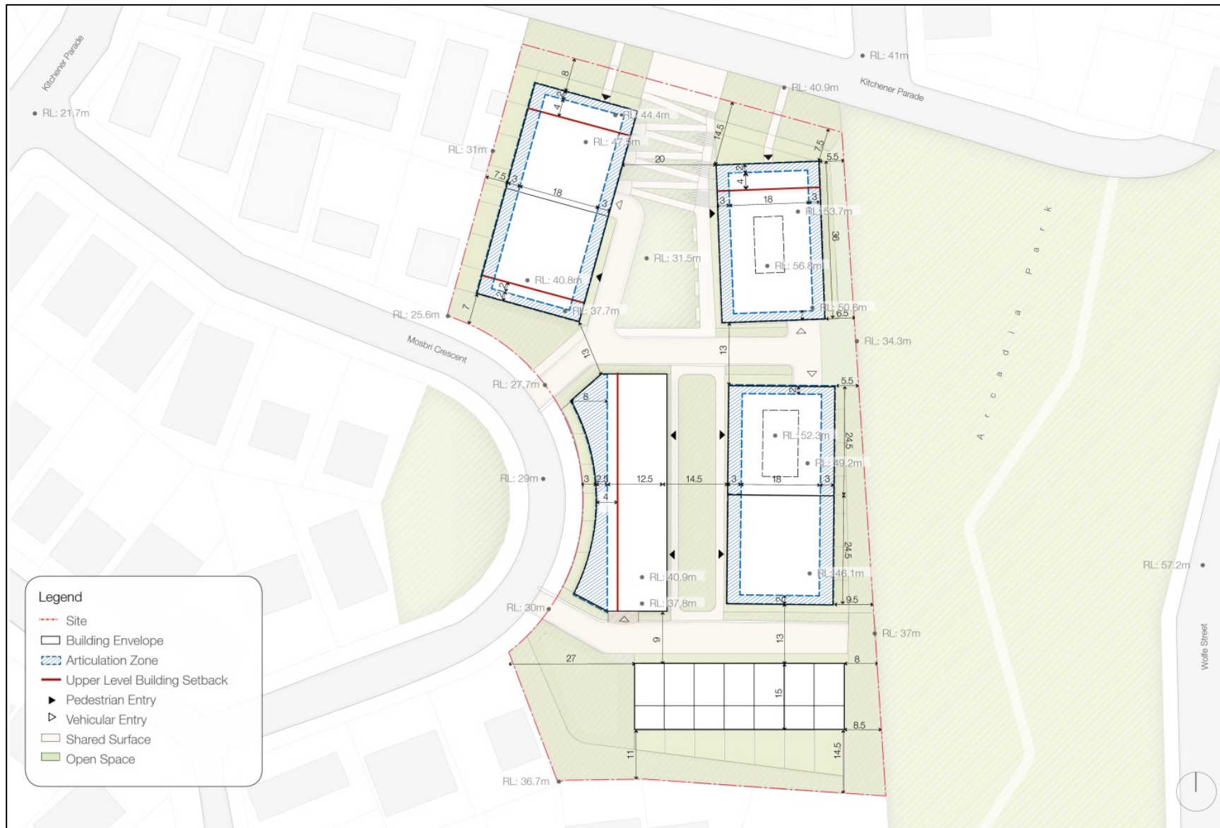
Map 3 – Building Setbacks
